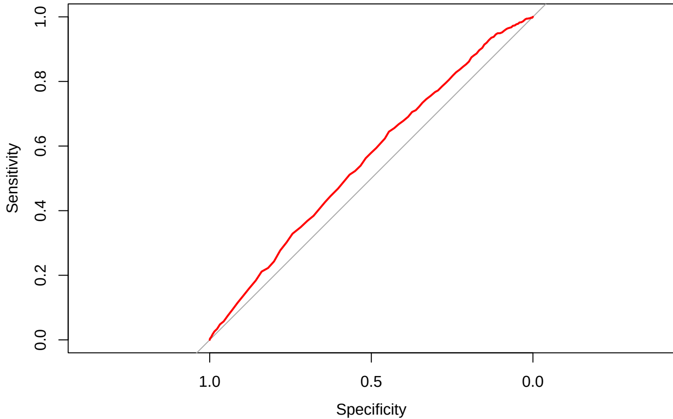
ROC-Kurve (Random Forest)
